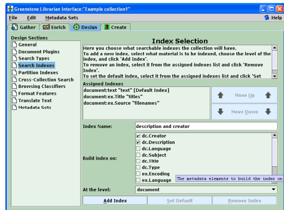
Figure 10. Adding a full-text-search index
